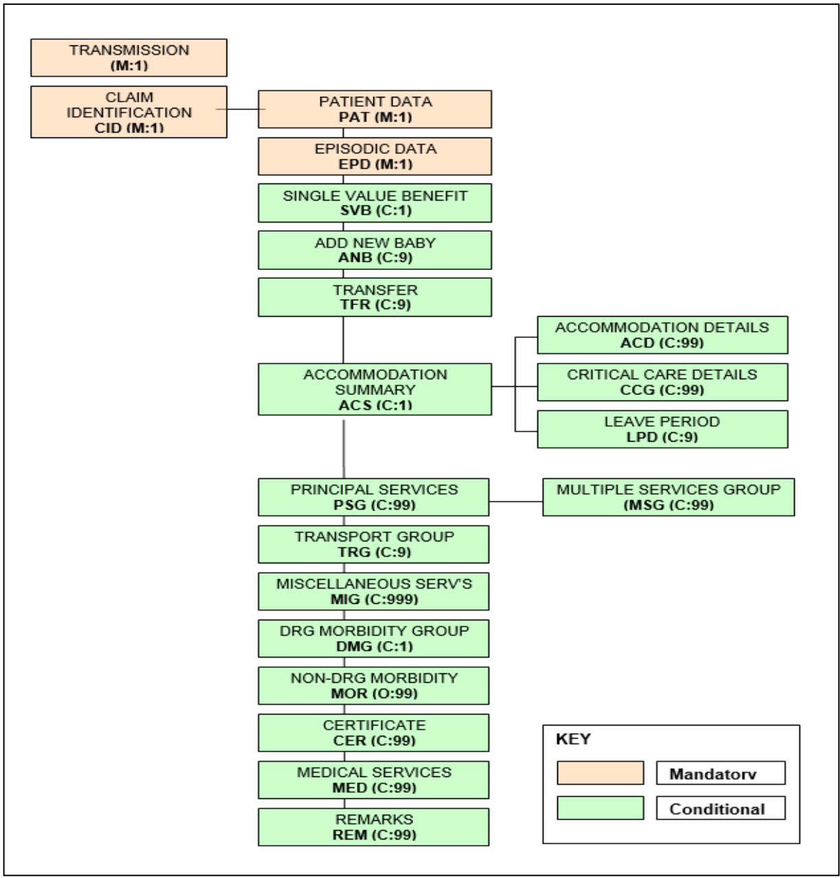
Figure 3: Hospital claim message example
